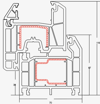
C70 CHAMFERED PROFILE
